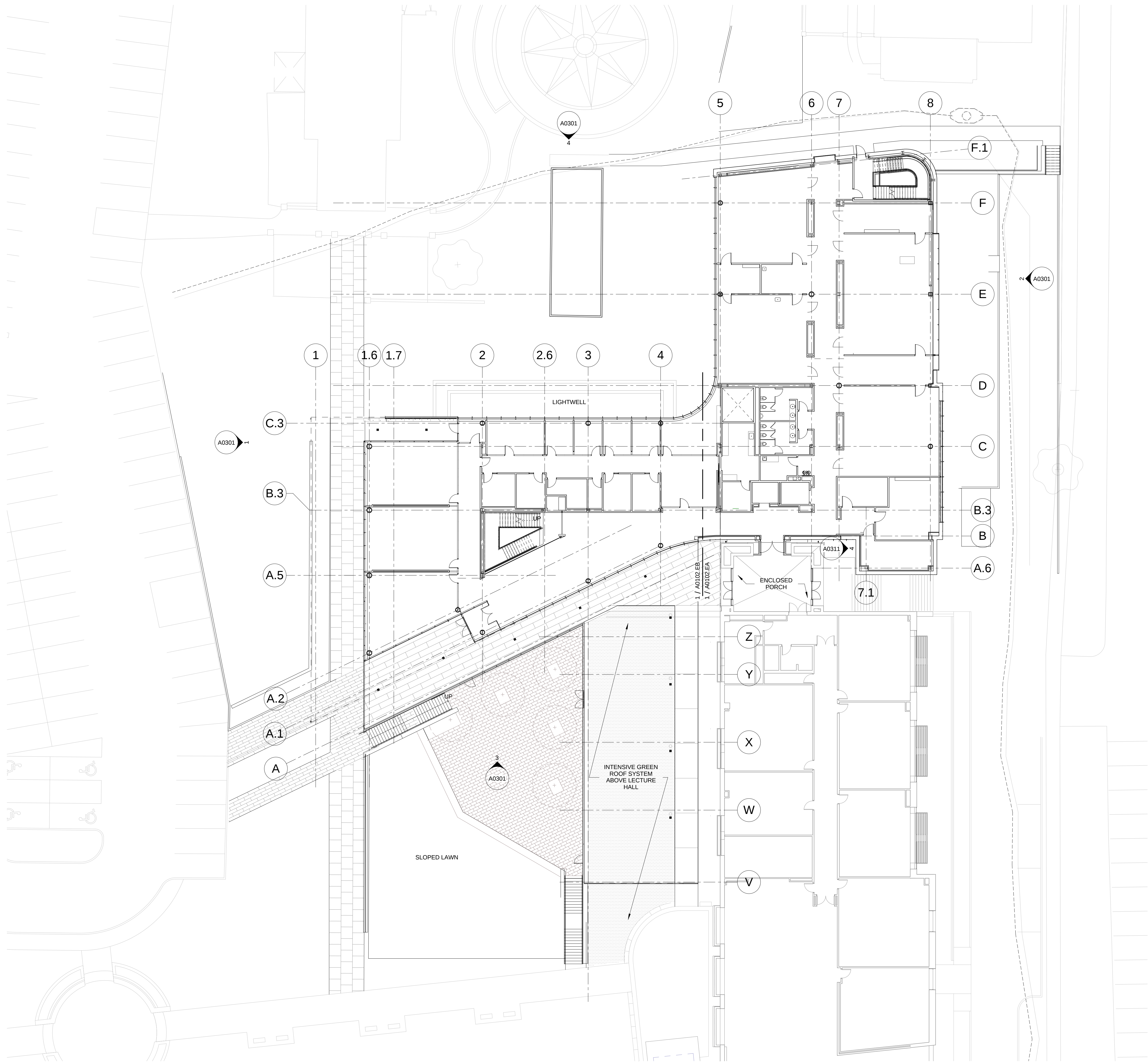
1 EXTERIOR - LEVEL 02 1/16" = 1'-0"
